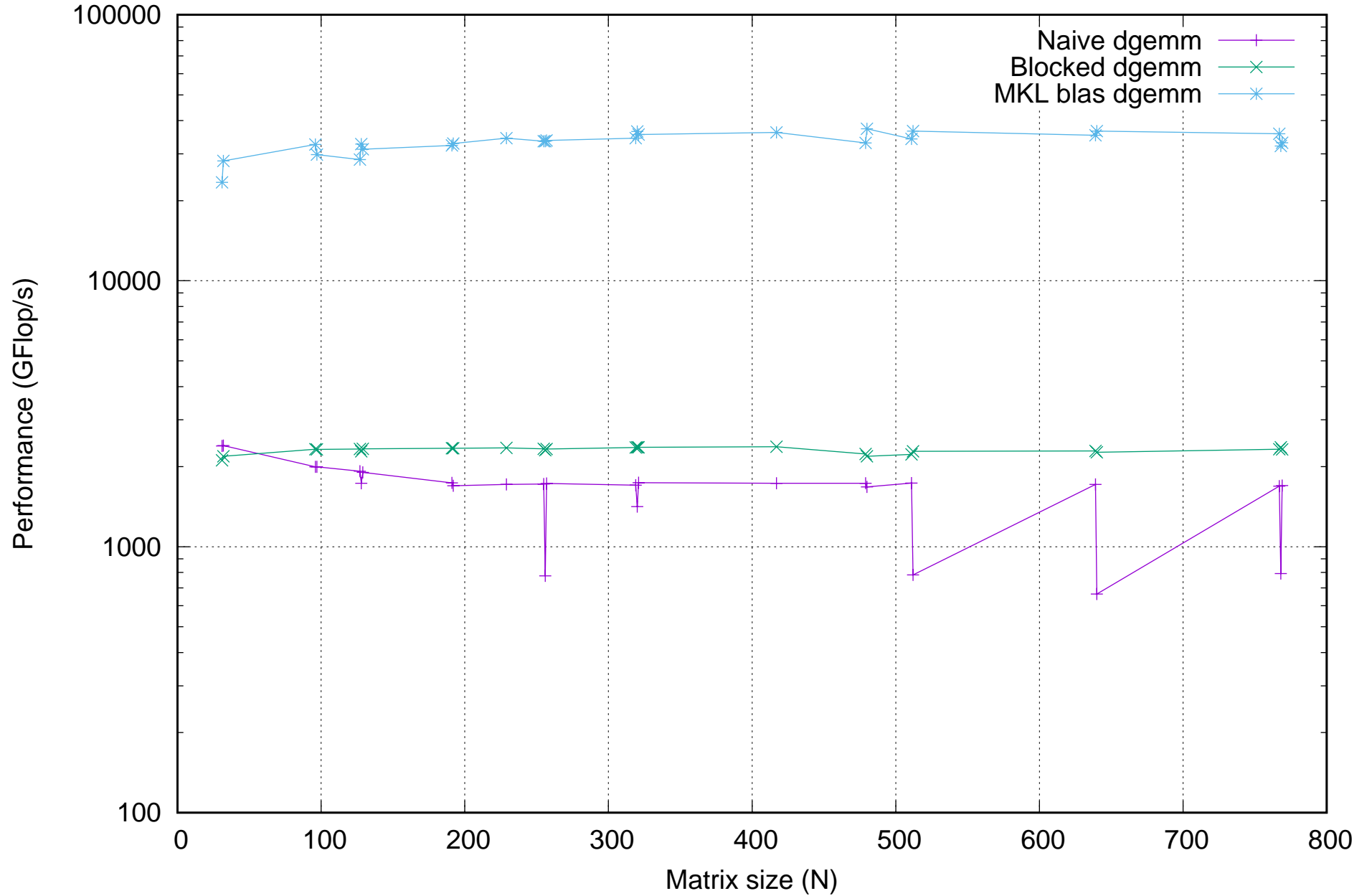
NxN matrix-matrix-multiplication on 4-Core Intel(R) Xeon(R) CPU E3-1585L v5 3.00GHz
