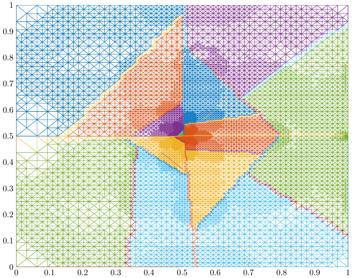
Inertial bisection for crack with n=16
