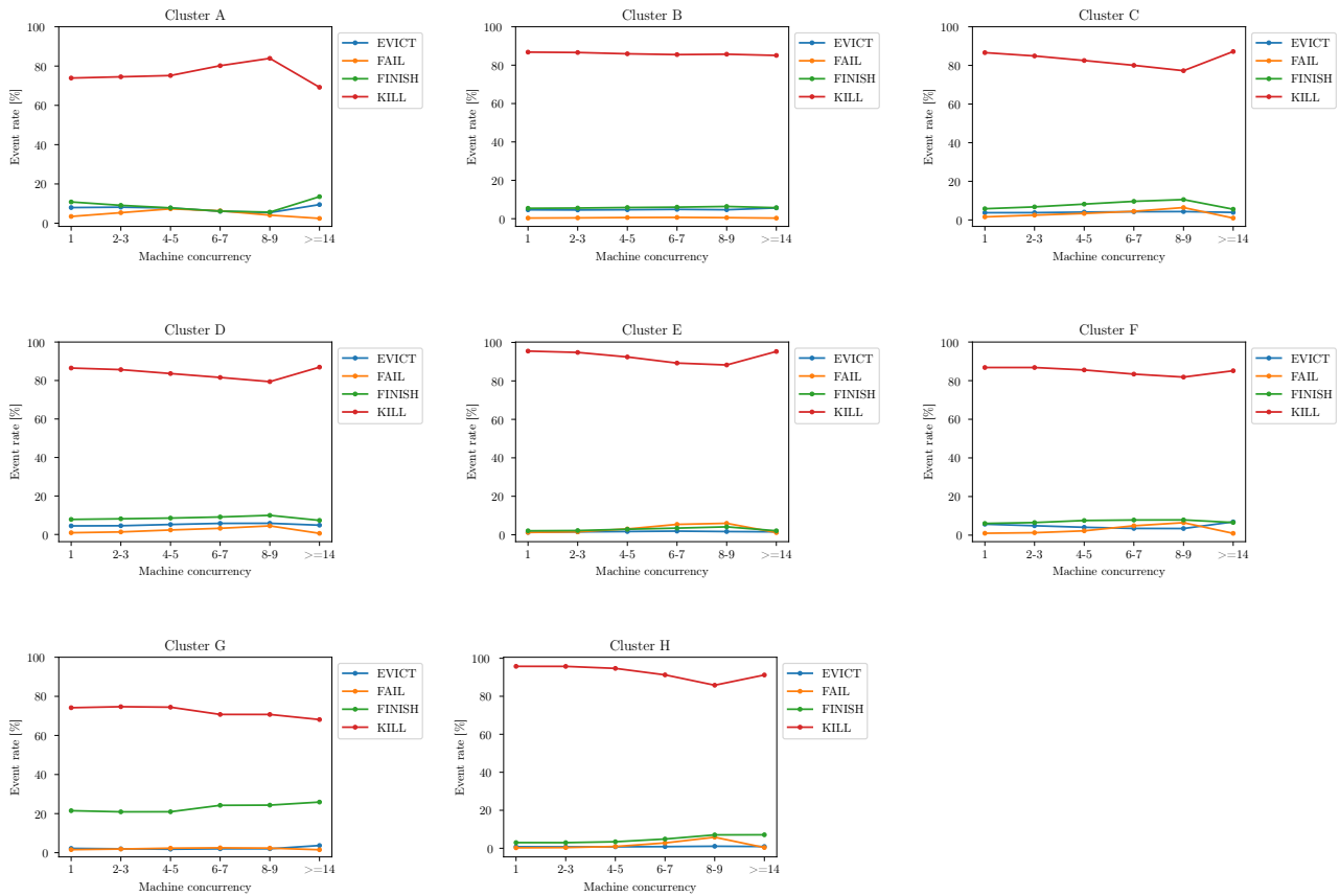
Figure 19. Task event rates vs. machine concurrency and final task termination in each 2019 cluster. Refer to figure 18 for the definition of “machine concurrency”.
