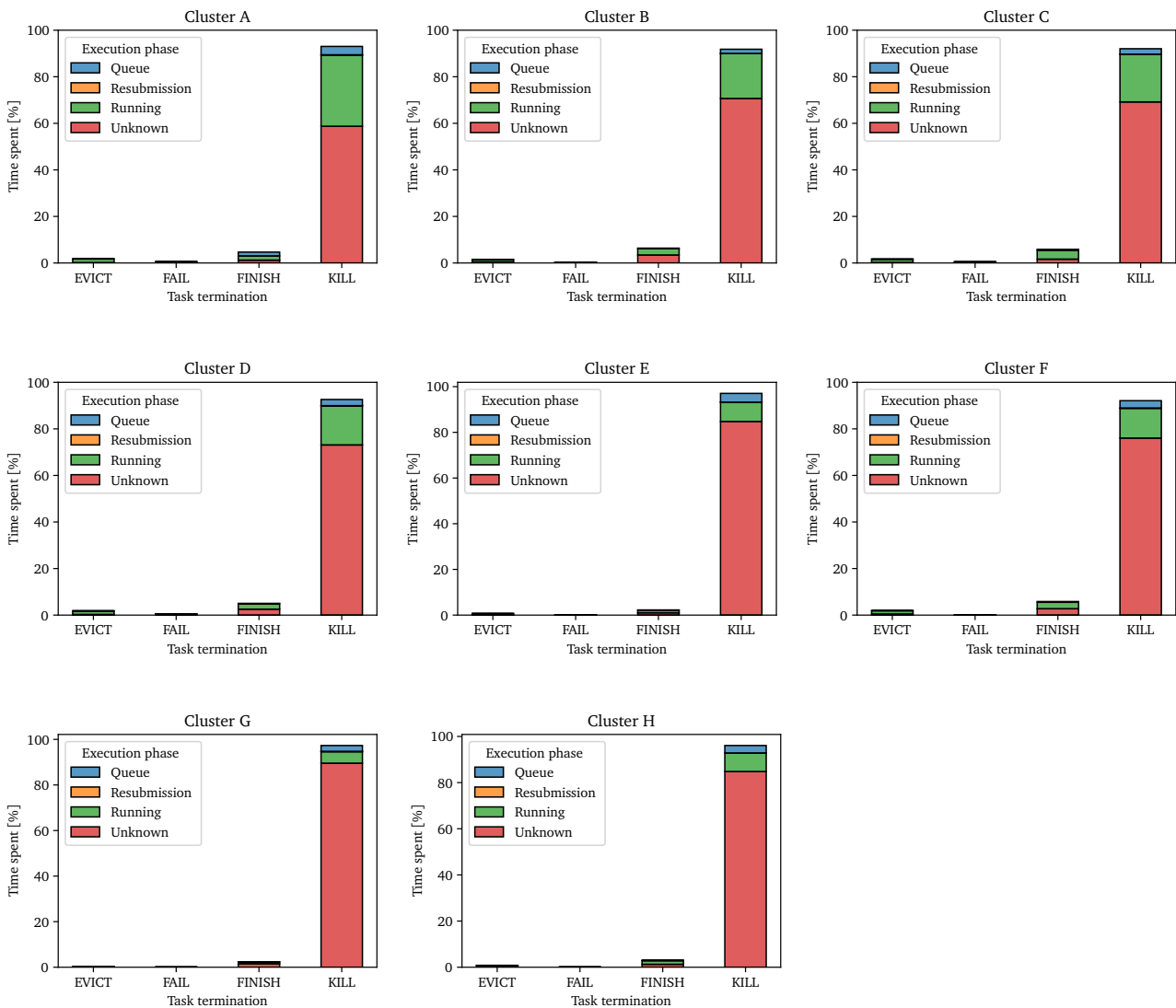
Figure 8. Relative task time spent in each execution phase w.r.t. clusters in the 2019 trace. Refer to Figure 6 for axes description.
