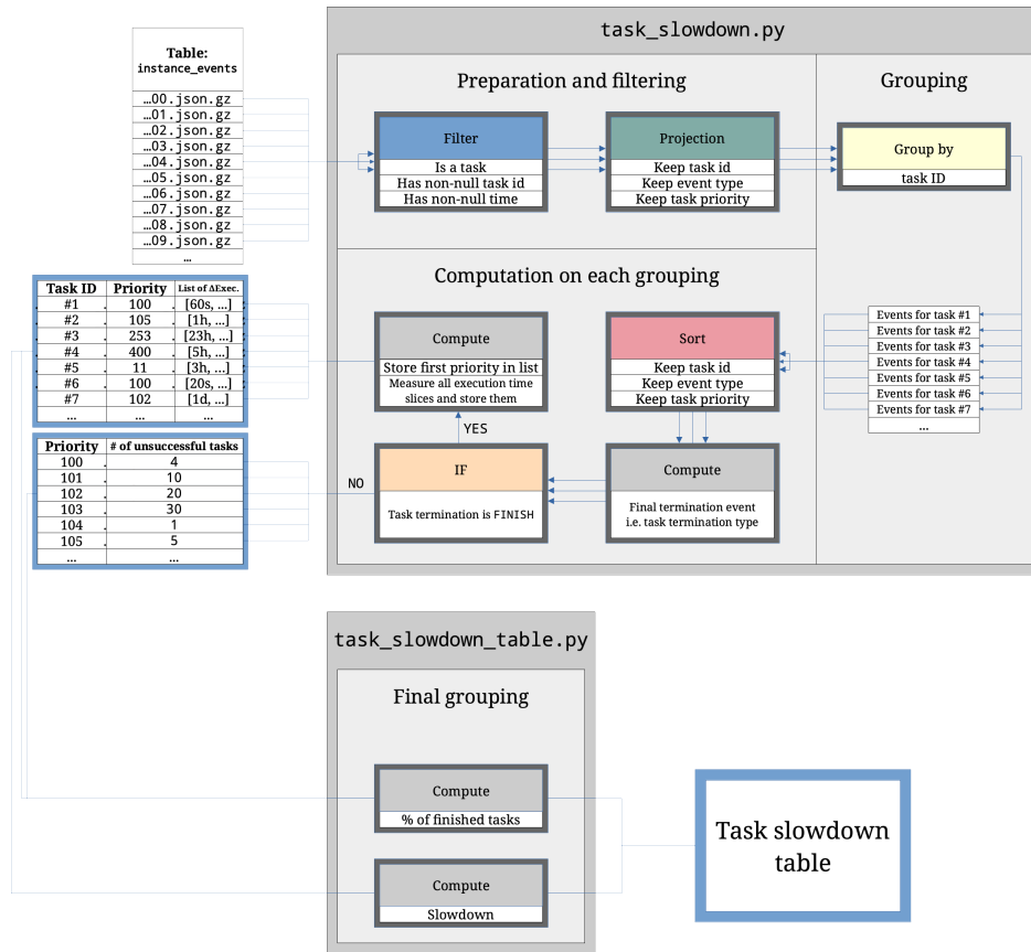
Figure 2. Diagram of the query scripts used for the “task slowdown” query
