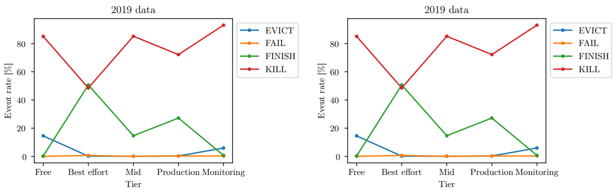
Figure 13. Task event rates vs. task priority and final task termination
