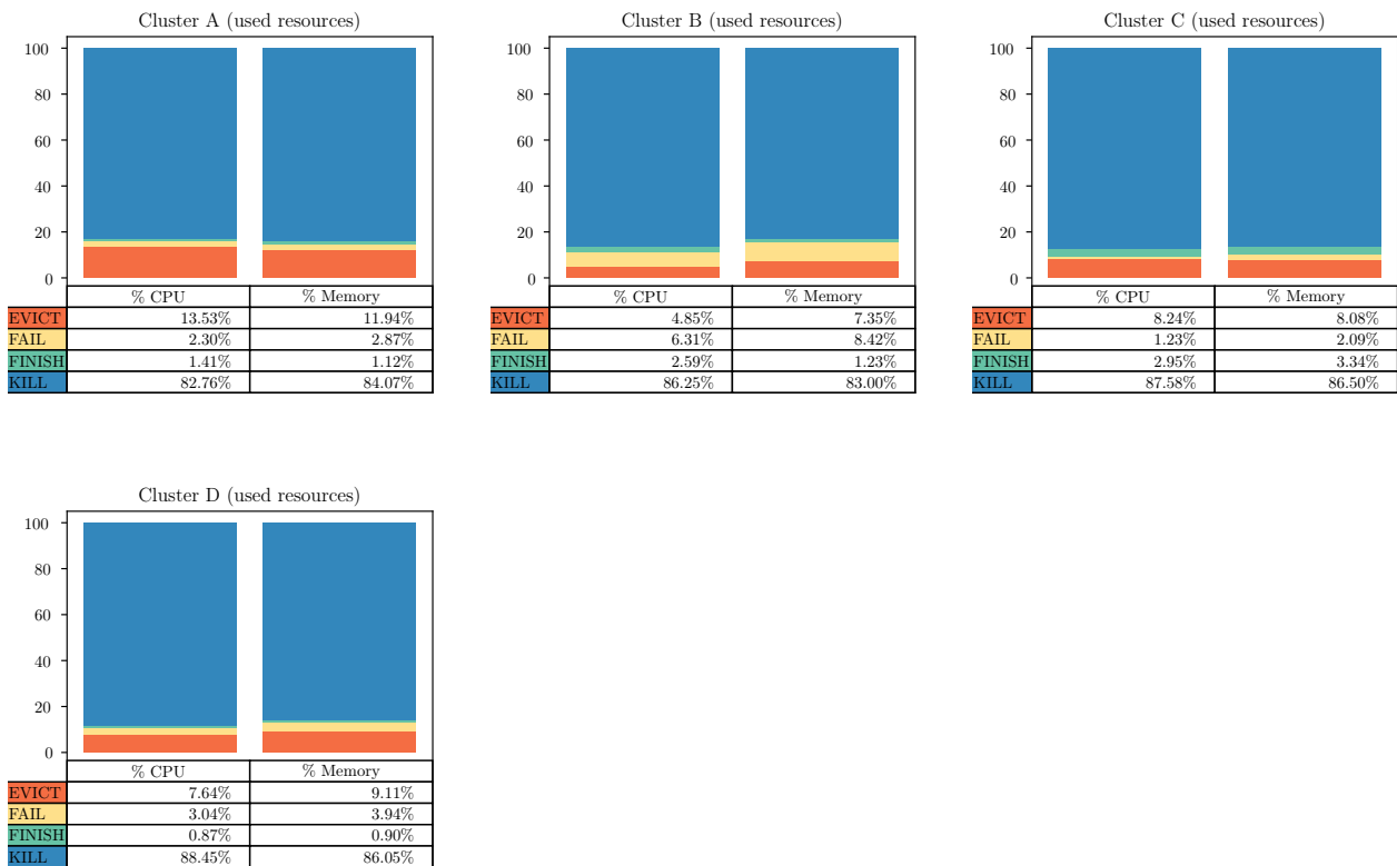
Figure 10. Percentages of CPU and RAM resources used by tasks w.r.t. task termination type for clusters A to D in 2019 traces. Refer to figure 11 for plot explanation.
