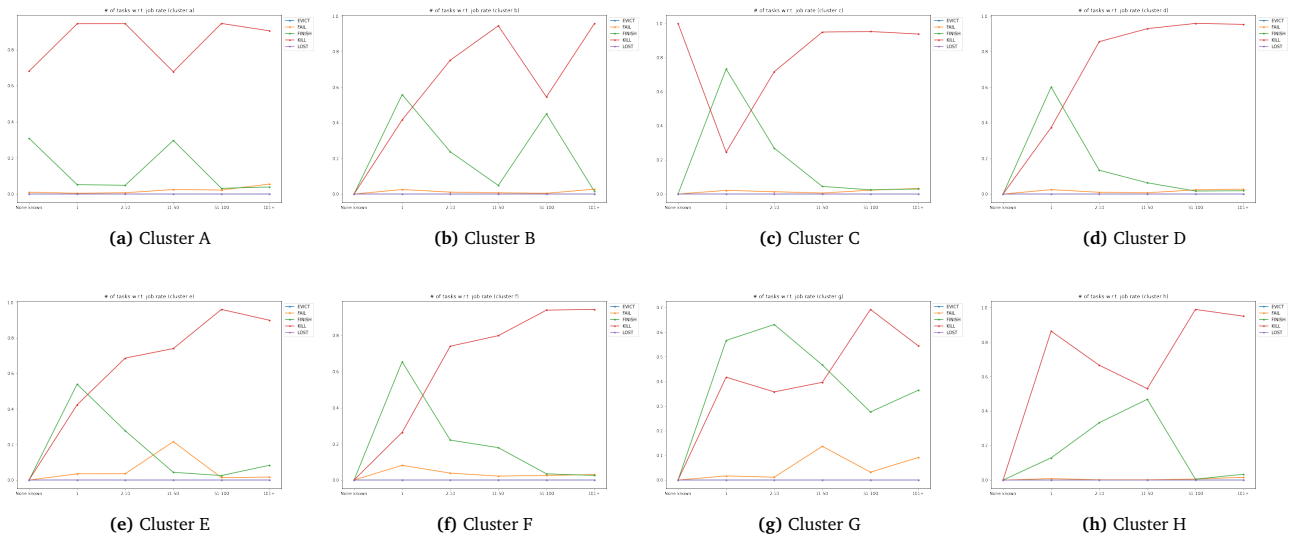
Figure 16. Job event rates vs. job size and final job termination
