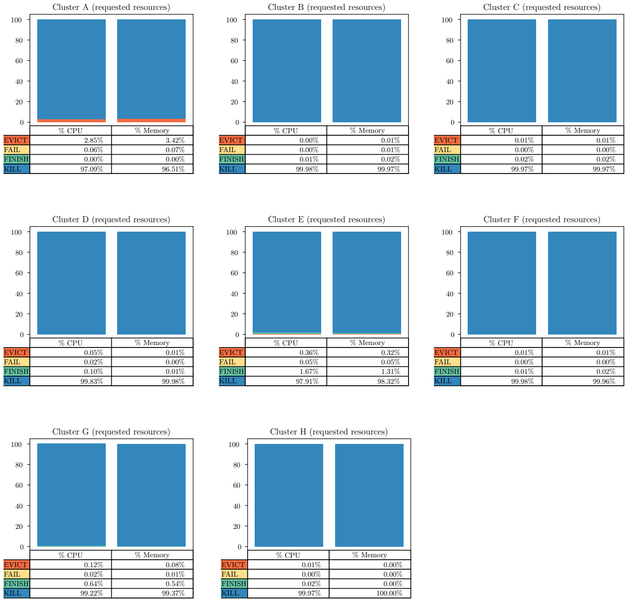
Figure 12. Percentages of CPU and RAM resources requested by tasks w.r.t. task termination type for in 2019 traces. Refer to figure 11 for plot explanation.
