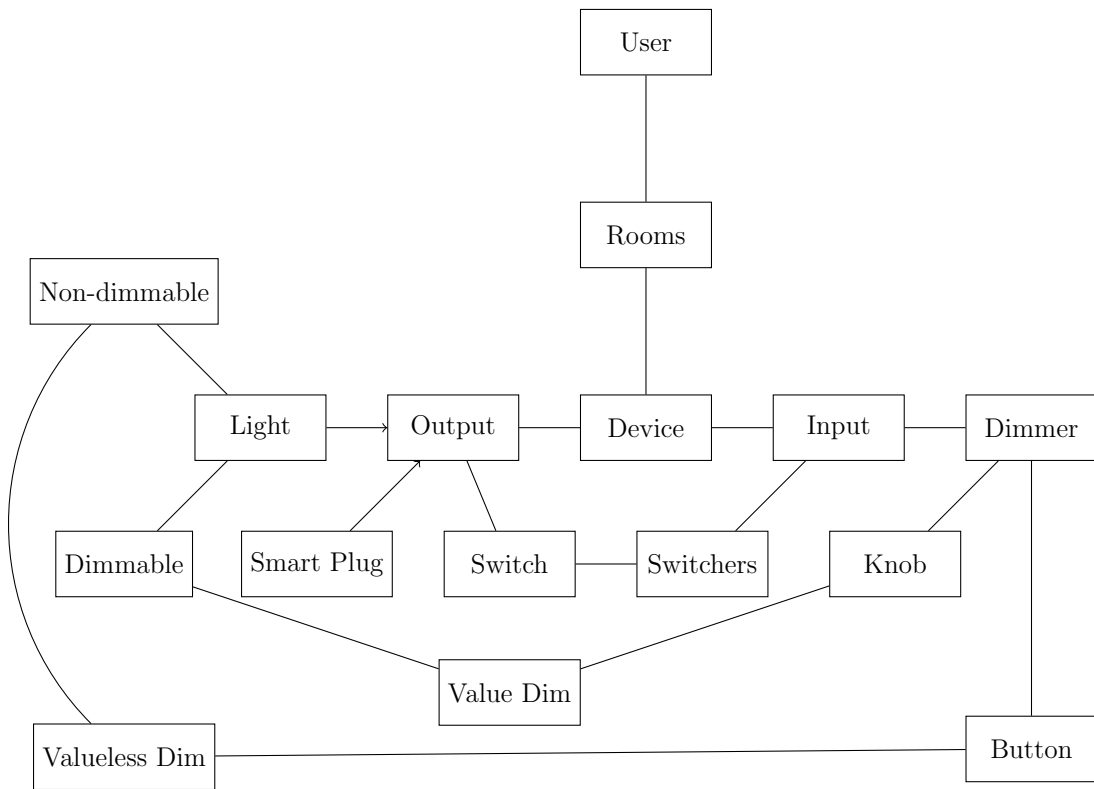
Entity Relationship Diagram for the SmartHut project
