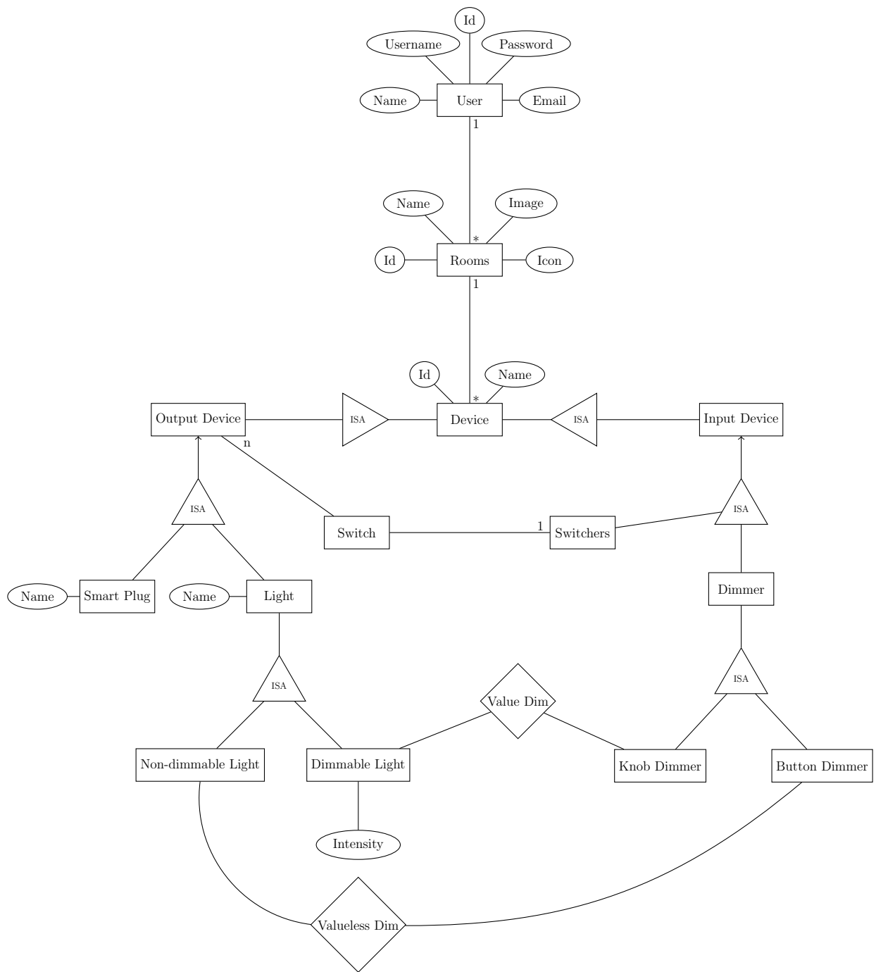
Entity Relationship Diagram for the SmartHut project
